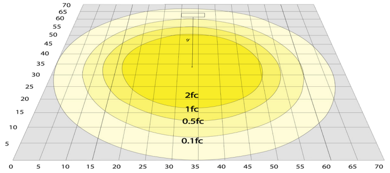
Simulation based on 4000K Area 70'x 70' Mounting Height: 9'
